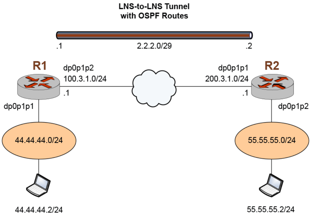
FIGURE 13 Sample LNS-to-LNS IPv4 tunnel with OSPF routes
