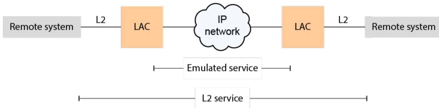
FIGURE 6 LAC-to-LAC tunneling reference model
