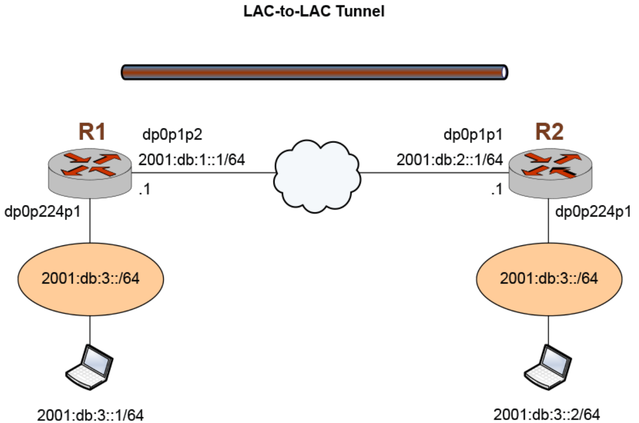
FIGURE 10 Sample LAC-to-LAC IPv6 tunnel
