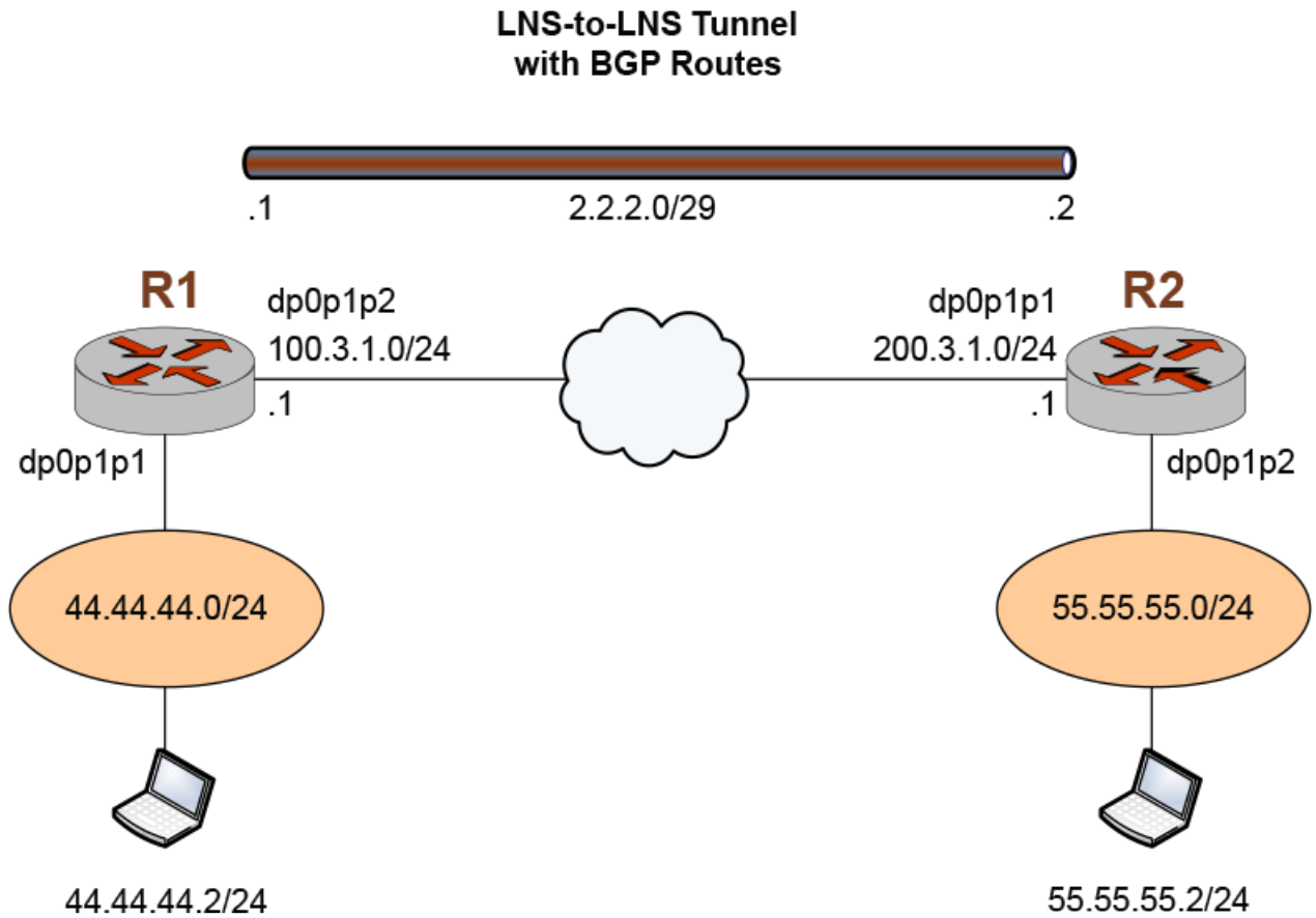
FIGURE 12 Sample LNS-to-LNS IPv4 tunnel with BGP routes
