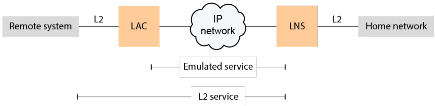
FIGURE 7 LAC-to-LNS tunneling reference model
