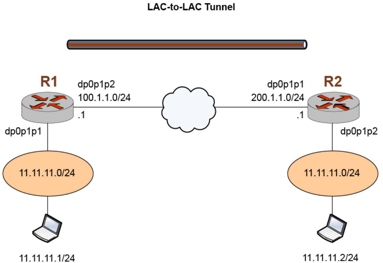
FIGURE 9 Sample LAC-to-LAC IPv4 tunnel
