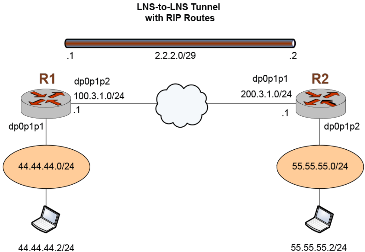
FIGURE 14 Sample LNS-to-LNS IPv4 tunnel with RIP routes
