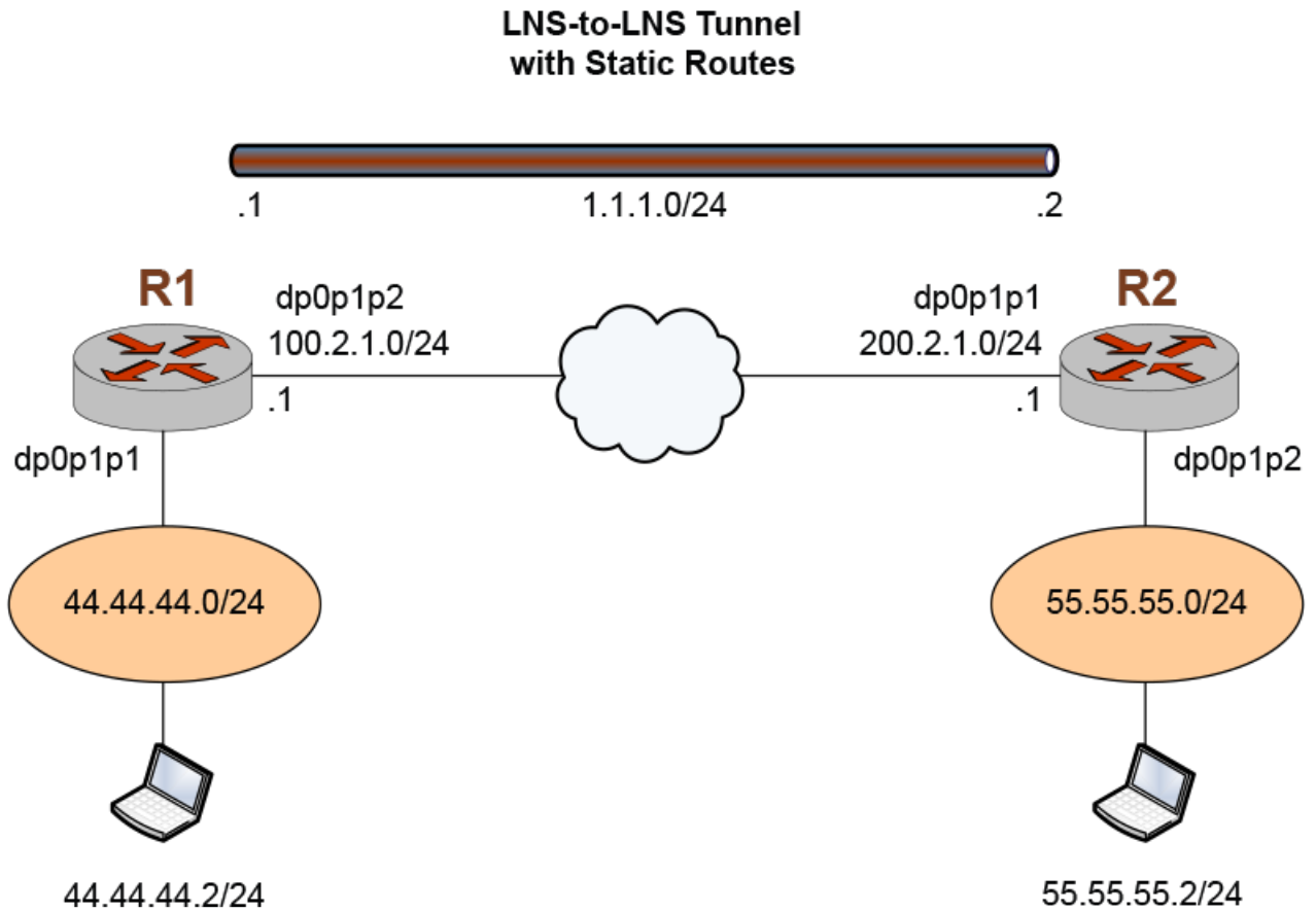
FIGURE 11 Sample LNS-to-LNS IPv4 tunnel
