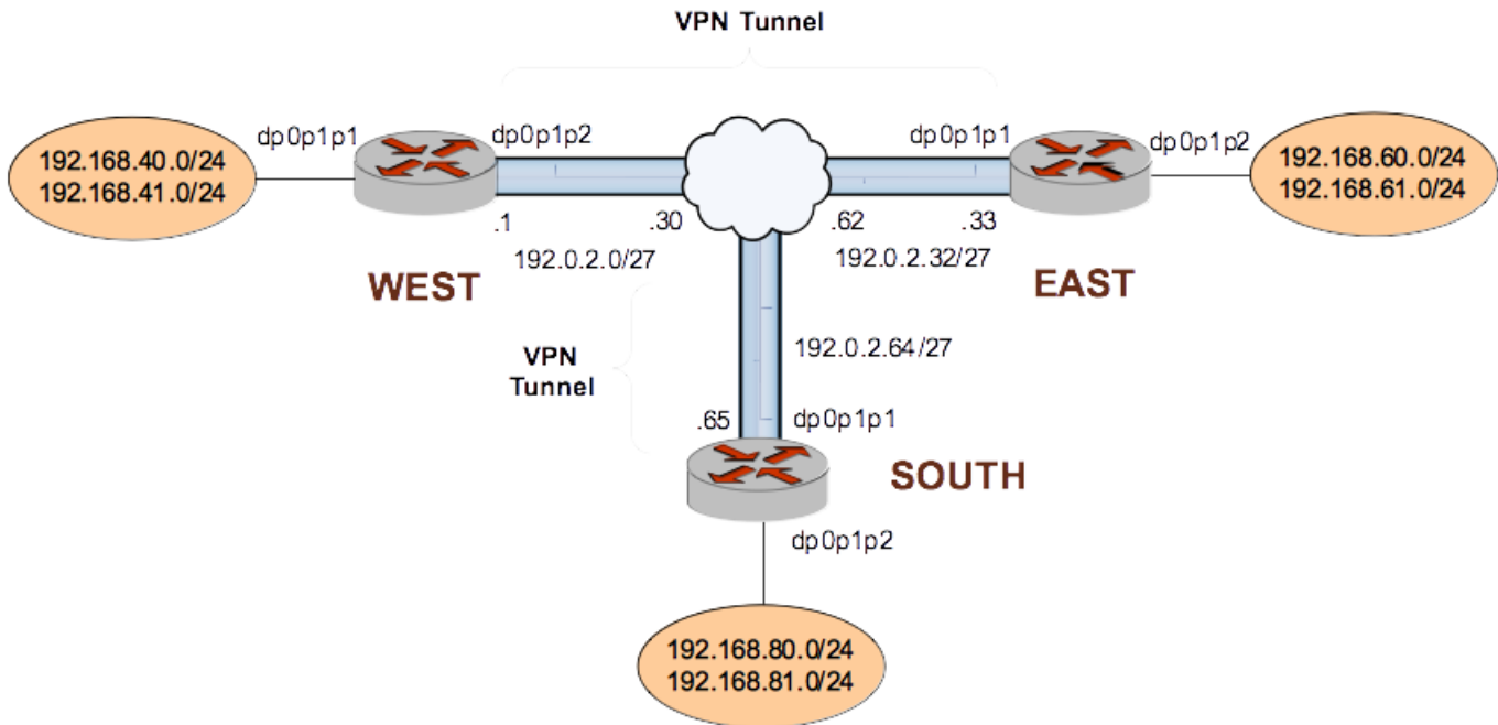
FIGURE 4 Multiple site-to-site tunnels between three gateways
