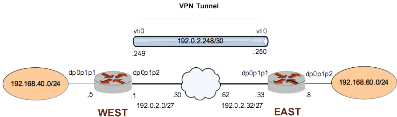
FIGURE 6 IPsec VPN connection with virtual tunnel interfaces
