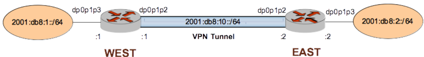
FIGURE 7 Basic site-to-site IPsec VPN connection over IPv6
