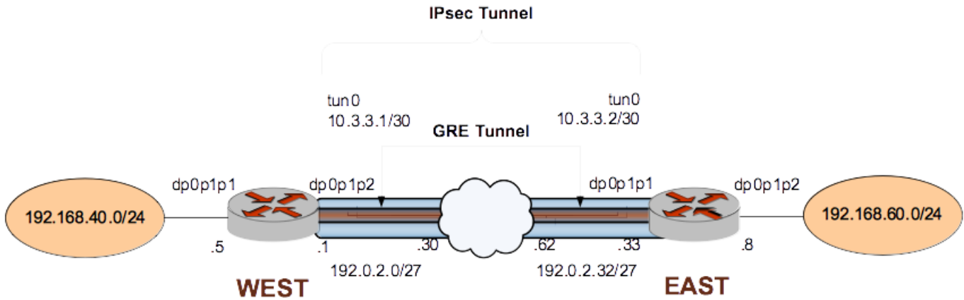
FIGURE 5 GRE tunnel protected by an IPsec tunnel
