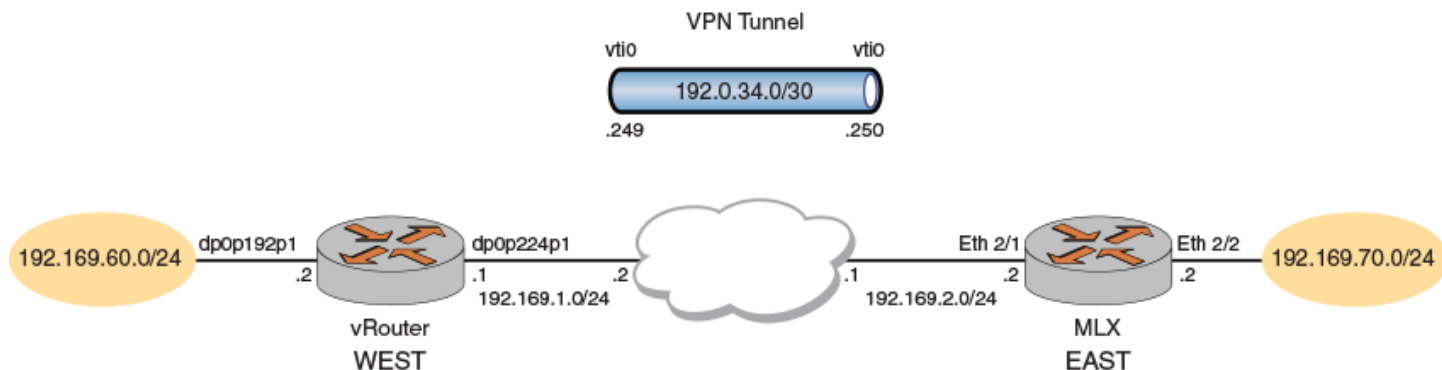
FIGURE 8 Virtual tunnel interface to an MLX router
