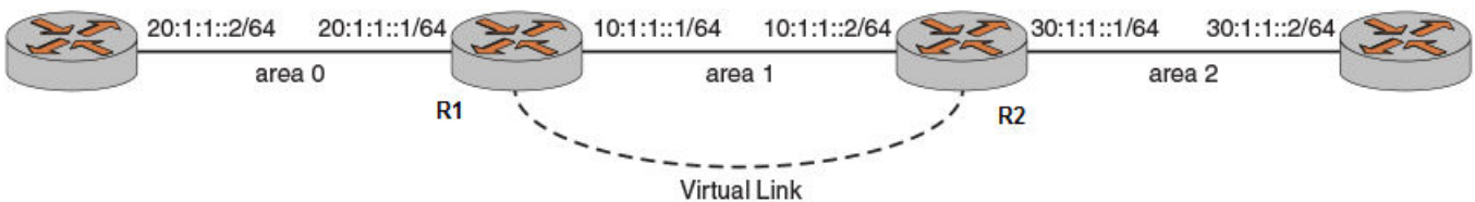
FIGURE 20 Configuring BFD for OSPFv3 on a virtual interface by using IPv6 addressing
