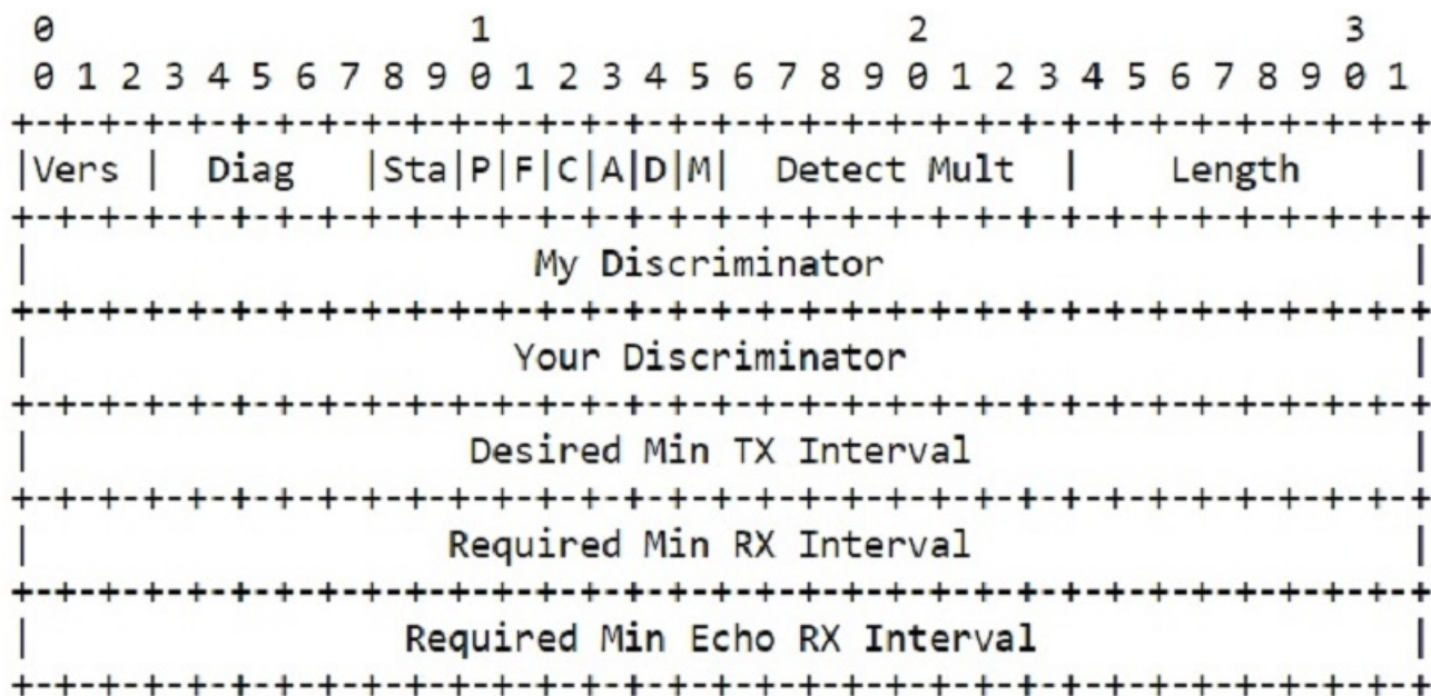
FIGURE 2 Format of a BFD control packet
