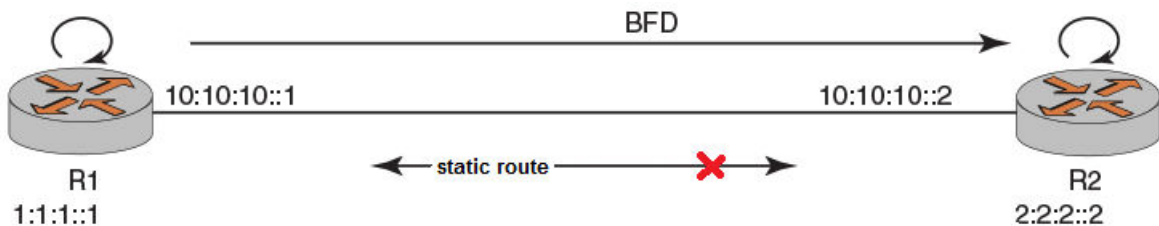
FIGURE 17 Configuring a BFD helper session by using IPv6 addressing
