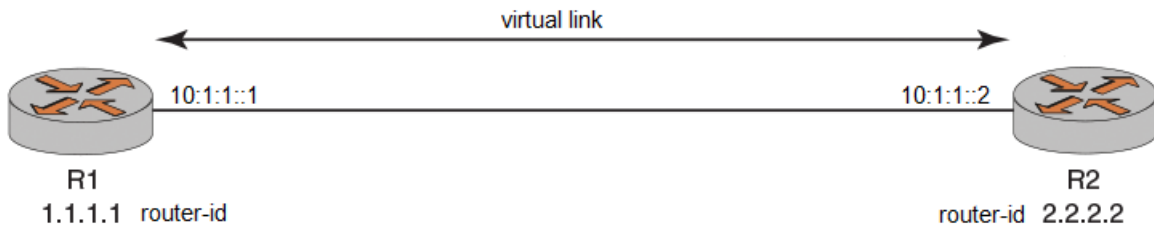
FIGURE 19 Configuring BFD for OSPFv3 on a virtual link by using IPv6 addressing
