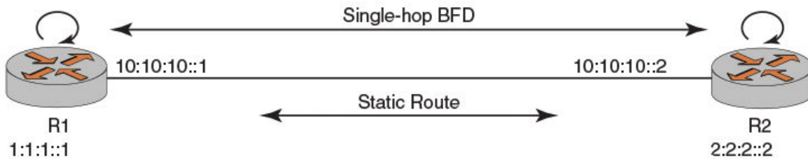
FIGURE 15 Configuring BFD for static route single hop by using IPv6 addressing
