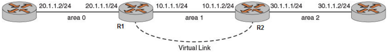
FIGURE 12 Configuring BFD for OSPFv2 on a virtual interface by using IPv4 addressing
