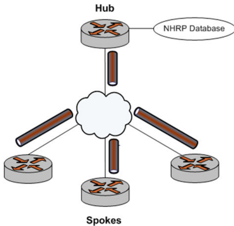
FIGURE 7 DMVPN
