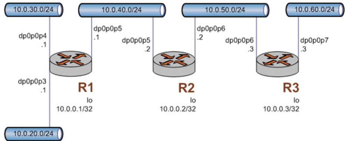
FIGURE 1 OSPF configuration diagram
