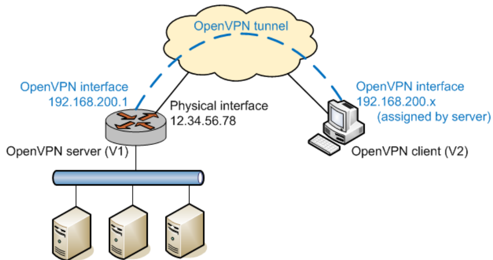
FIGURE 5 Client-server mode
