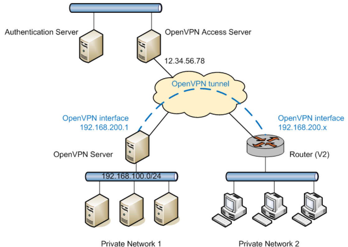
FIGURE 3 Client-side access to OpenVPN access server
