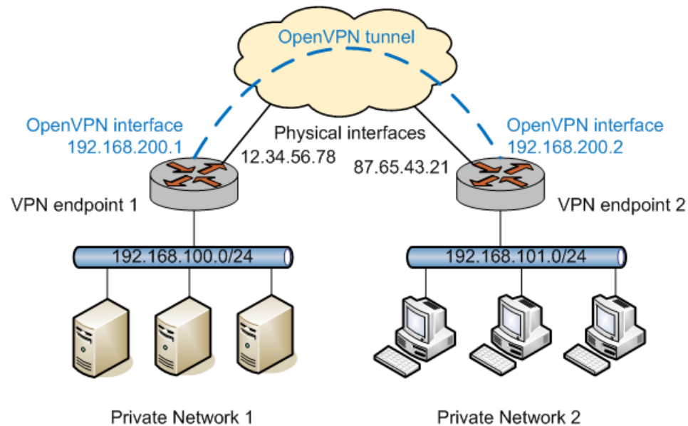
FIGURE 1 Site-to-site operation
