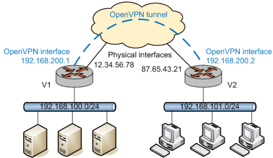
FIGURE 4 Site-to-site VPN with preshared secret
