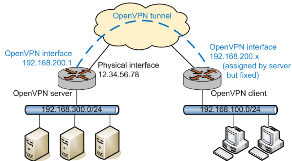
FIGURE 7 Client-server mode
