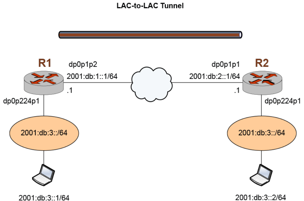
FIGURE 10 Sample LAC-to-LAC IPv6 tunnel
