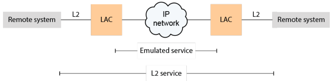
FIGURE 6 LAC-to-LAC tunneling reference model
