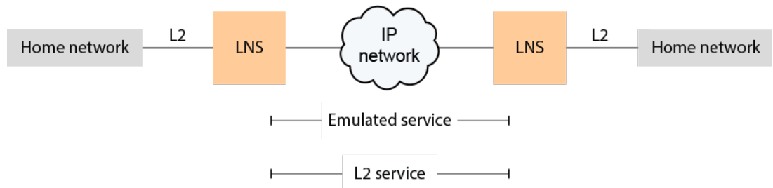
FIGURE 8 LNS-to-LNS tunneling reference model
