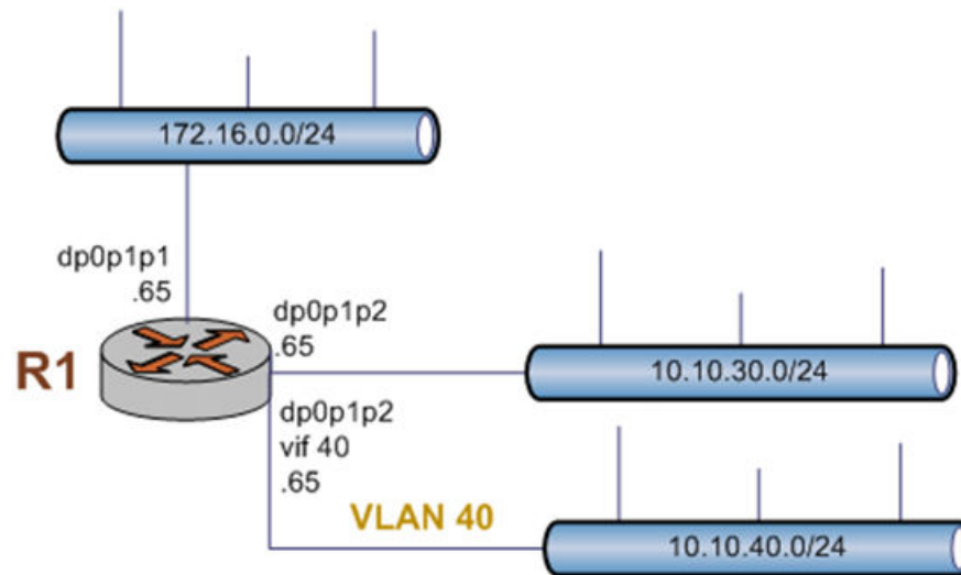
FIGURE 4 VLAN configuration
