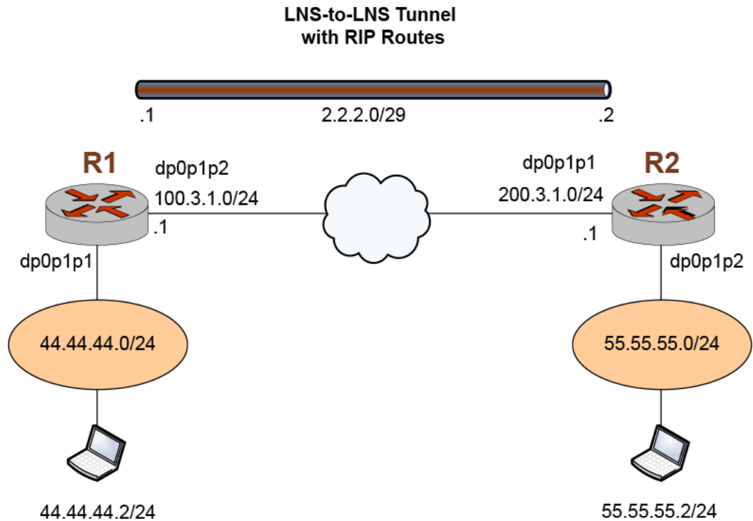
FIGURE 14 Sample LNS-to-LNS IPv4 tunnel with RIP routes
