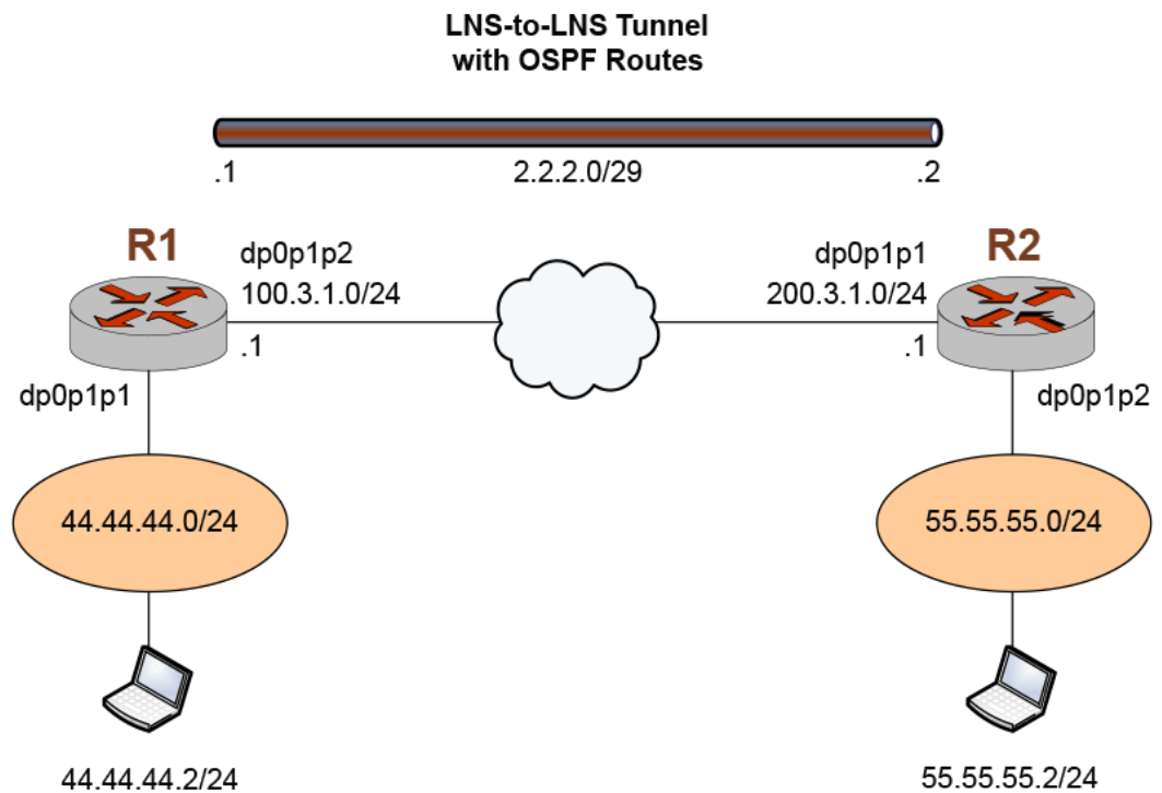
FIGURE 13 Sample LNS-to-LNS IPv4 tunnel with OSPF routes
