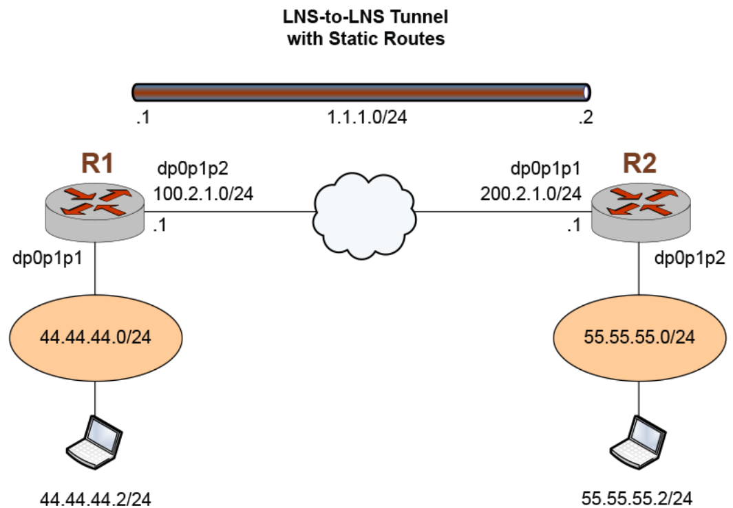
FIGURE 11 Sample LNS-to-LNS IPv4 tunnel
