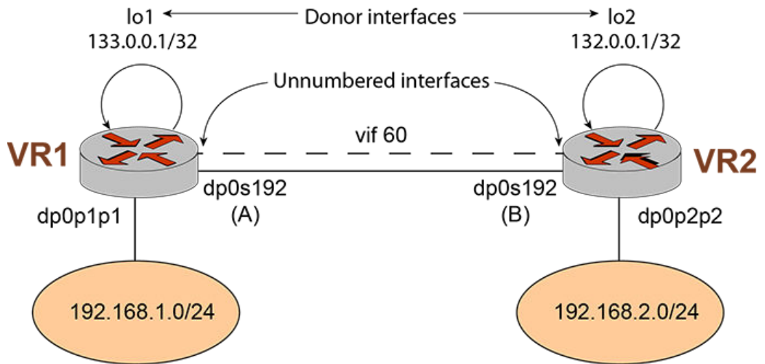
FIGURE 5 Configuring IP unnumbered interfaces
