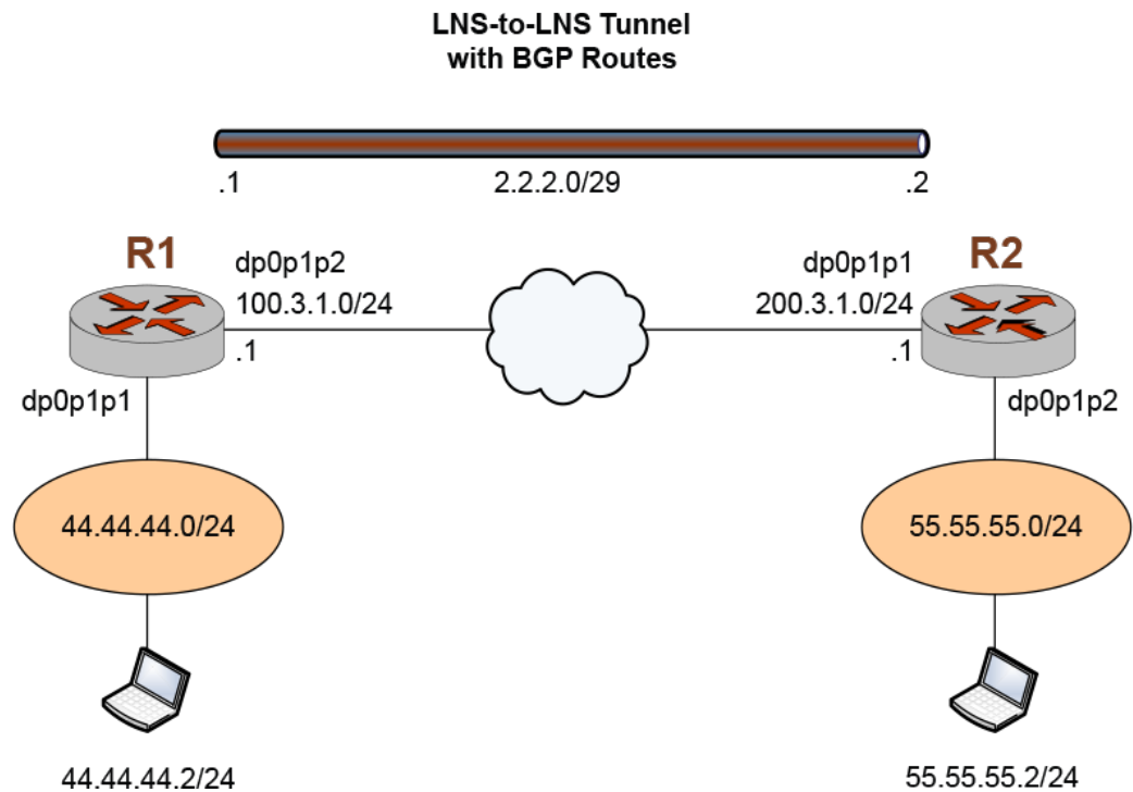
FIGURE 12 Sample LNS-to-LNS IPv4 tunnel with BGP routes
