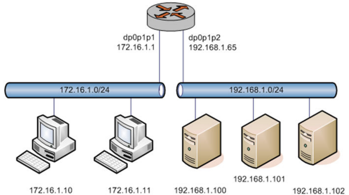
FIGURE 4 Excluding an address
