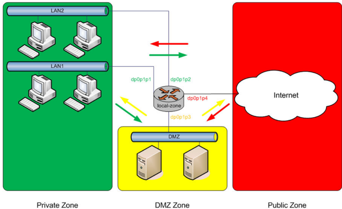
FIGURE 2 Zone-based firewall overview
