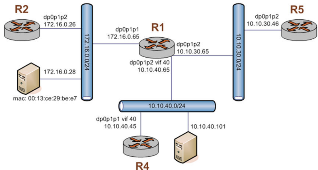
FIGURE 3 Firewall: sample configuration
