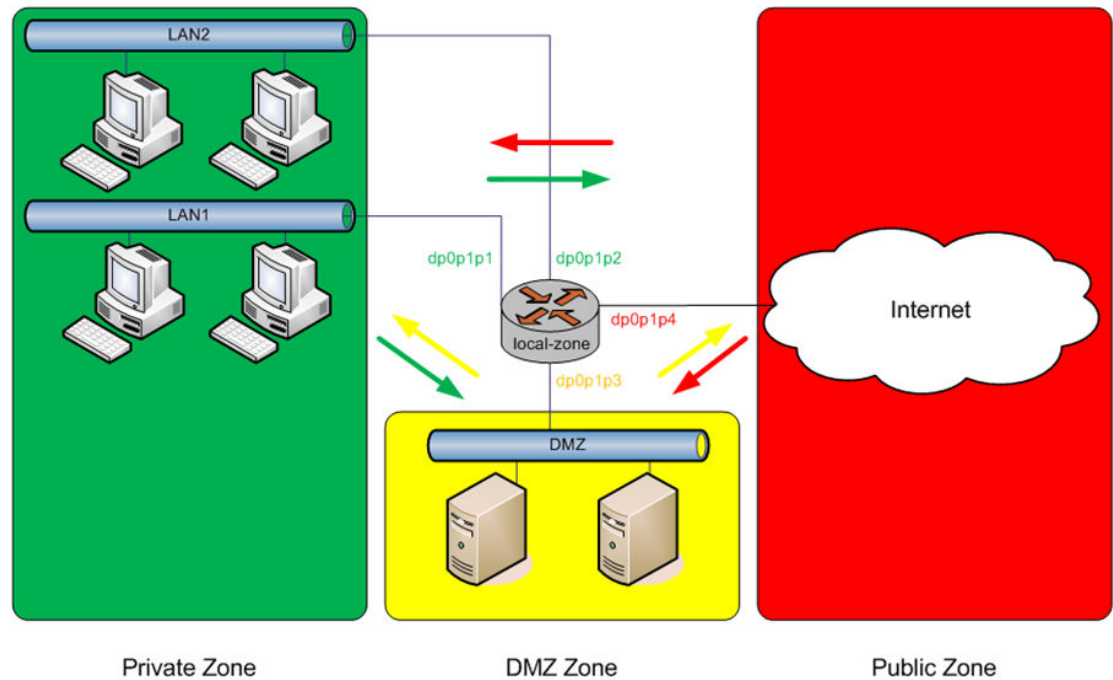
FIGURE 5 Zone-based firewall configuration
