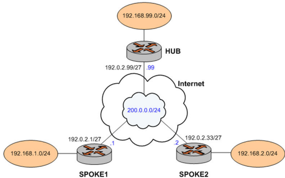
FIGURE 2 Basic mGRE tunnel network
